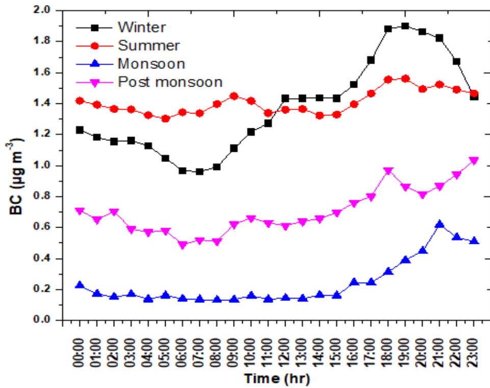
Fig. 3. Diurnal variation of BC during 2017
