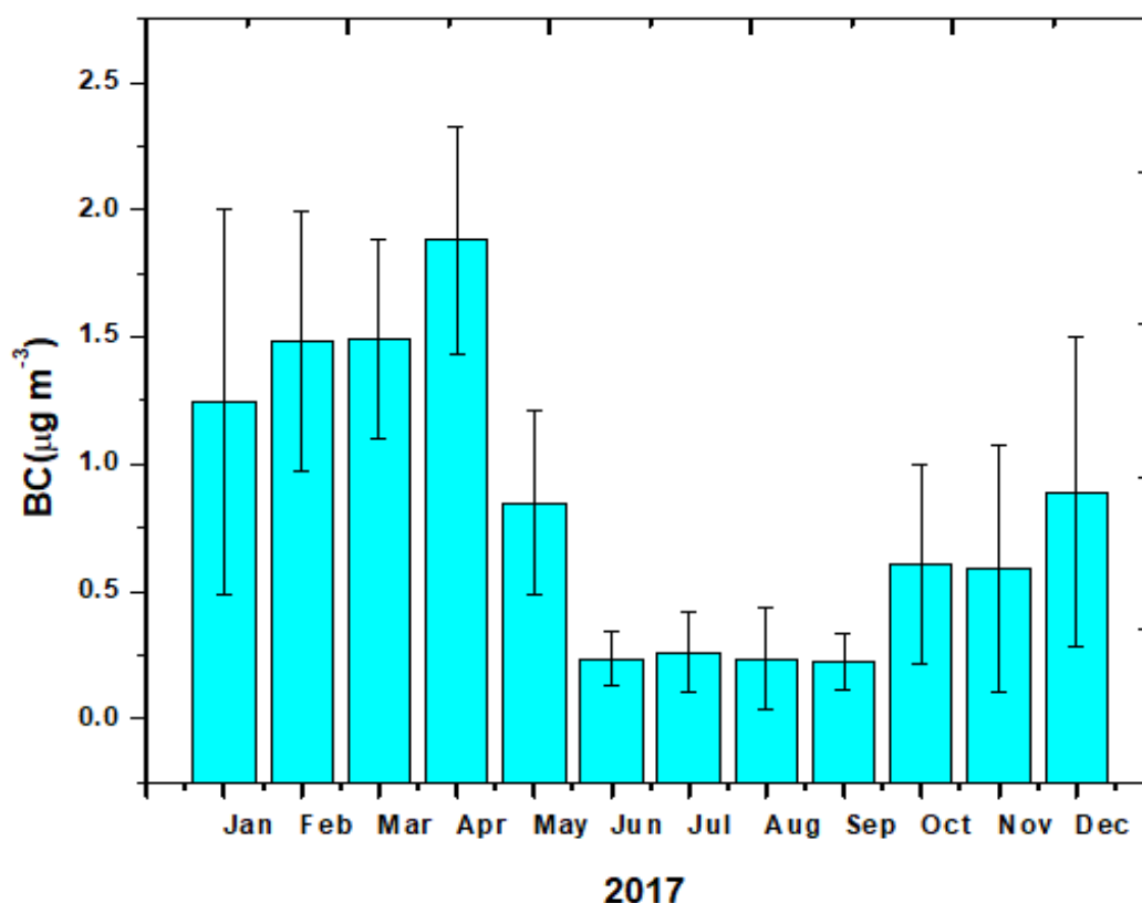
Fig. 2. Monthly variation of BC aerosol during 2017
