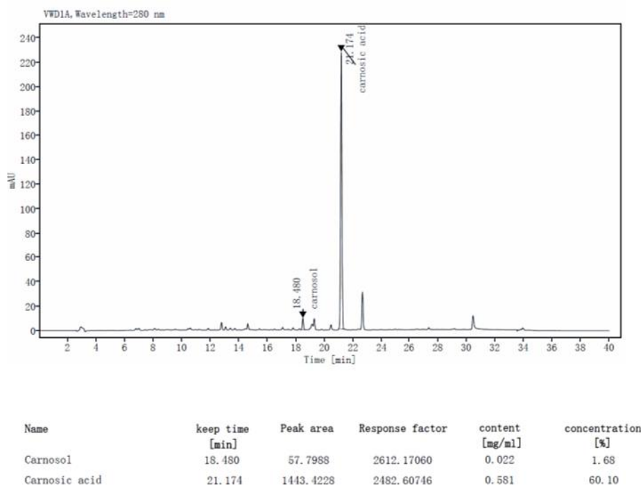
Graph 2. 60% standard peak of Carnosic acid (from Yangee Biotech China)
