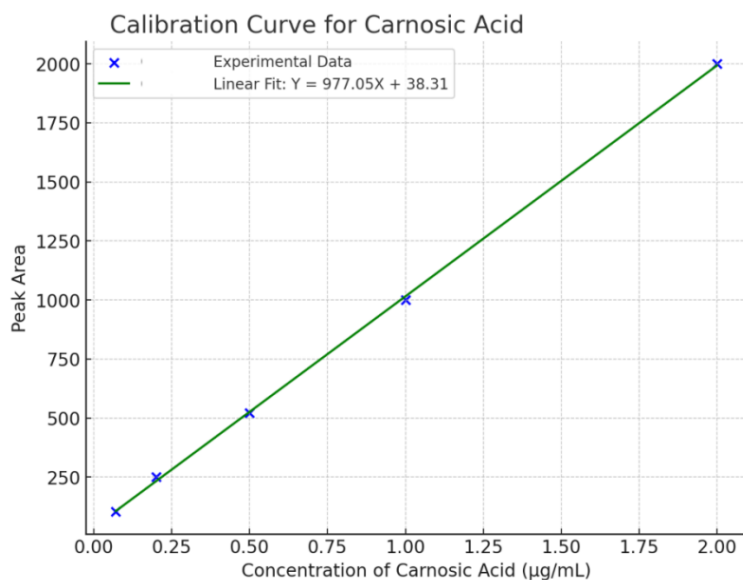
Graph 1. Calibration curve from experimental data
