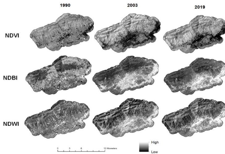
Fig. 5. Biophysical parameters (NDVI, NDBI, and NDWI) in 1990, 2003 and 2019
