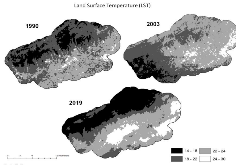
Fig. 4. Land surface temperature (LST) of Itanagar wildlife sanctuary in 1990, 2003 and 2019.
