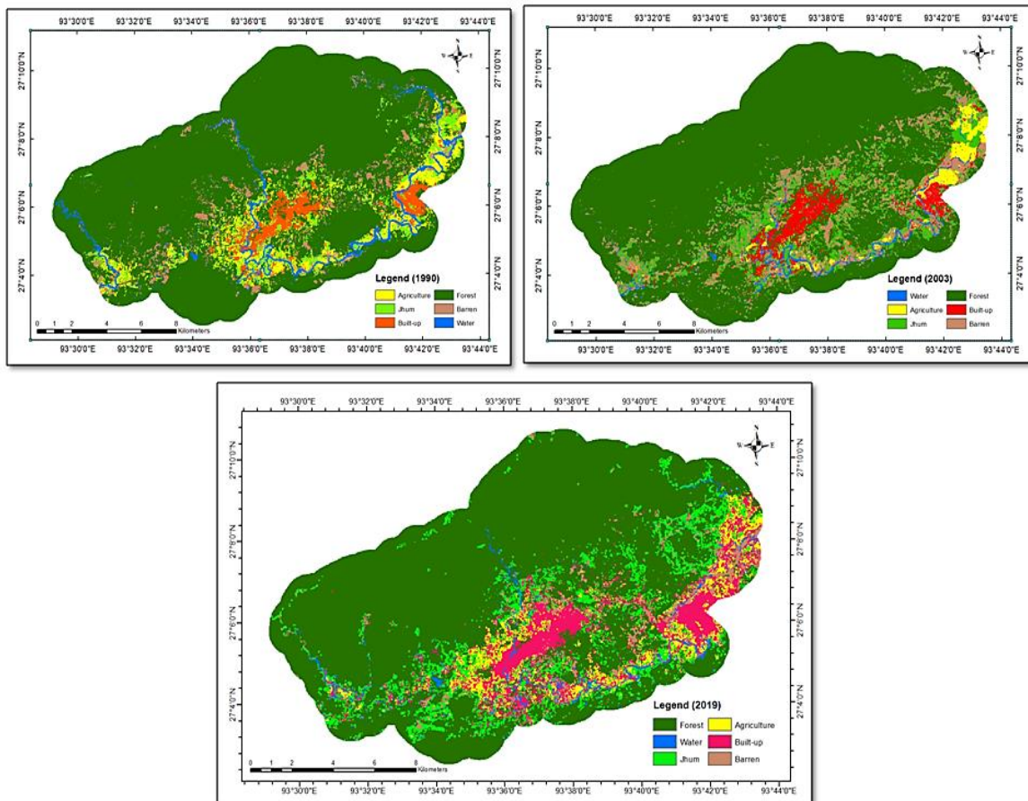
Fig. 3. LULC of Itanagar Wildlife Sanctuary in 1990, 2003 and 2019.
