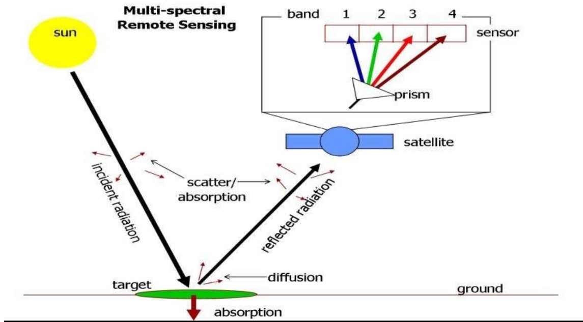
Fig. 3. Remote sensor
