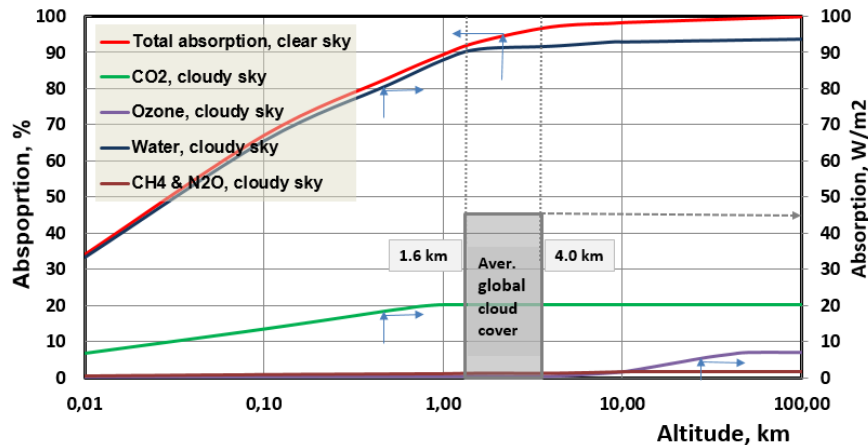
Fig. 6. The absorption effects of GH gases in the clear and cloudy sky conditions. The altitude axis is logarithmic
