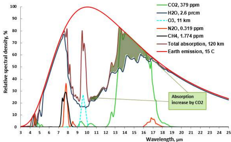
Fig. 3. The absorption band Graphs of GH gases in the AGA05 atmosphere. The green shaded areas indicate a total warming impact of CO 2 of concentration of 379 ppm
