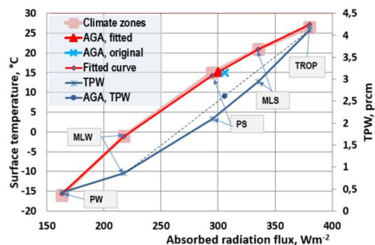
Fig. 1. The relationship between the absorption fluxes, temperatures, and water contents of different climate zones. The climate zones of the curves starting from the left corner are PW, MLW, PS, MLS, TROP. The temperatures and TPW values are from the climate profiles of Spectral Calculator [1]
