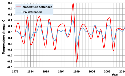
Fig. 5. The detrended graphs of temperature and TPW values
