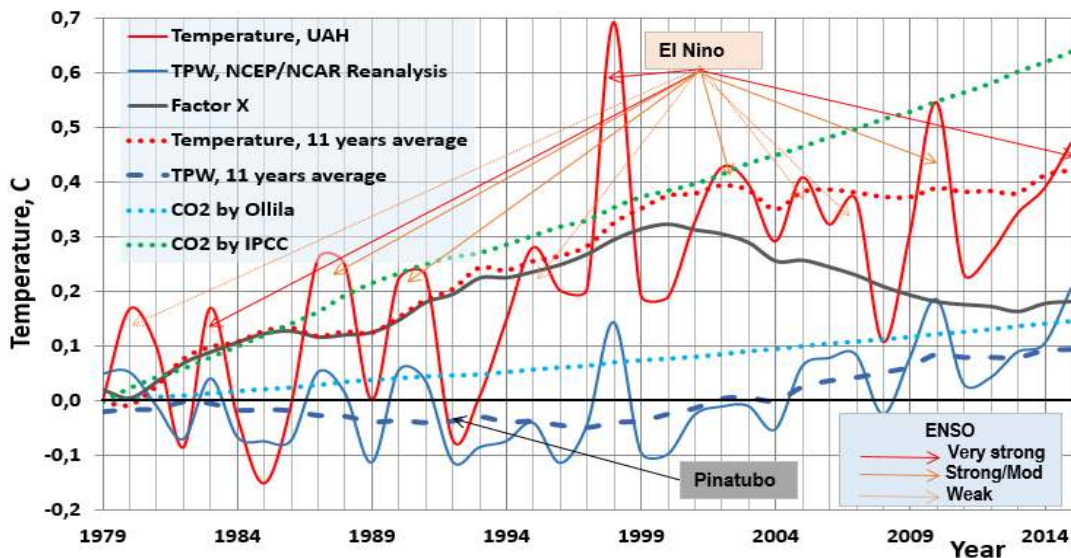
Fig. 4. The temperature trend from according to UAH [22] and the major warming factors, which are absolute humidity and CO 2 . The variable labelled “Factor X” is the difference between the measured average temperature and the warming impacts of CO 2 by Ollila [6]. El Niño events are marked as to the strengths and they are followed by La Niña events which are not marked
