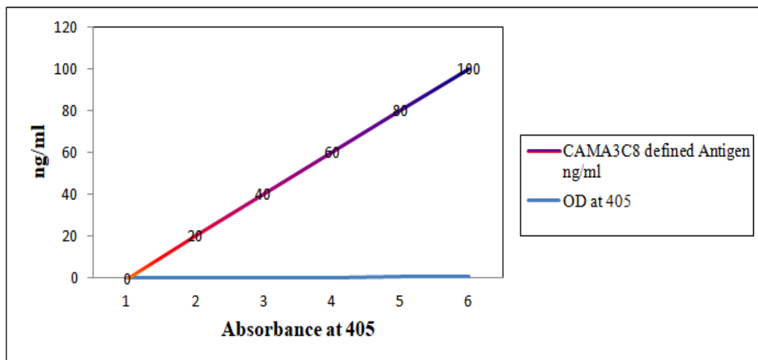
Fig. 1. Standard Curve for CAMA3C8 defined antigen (ng/ml) levels by ELISA
