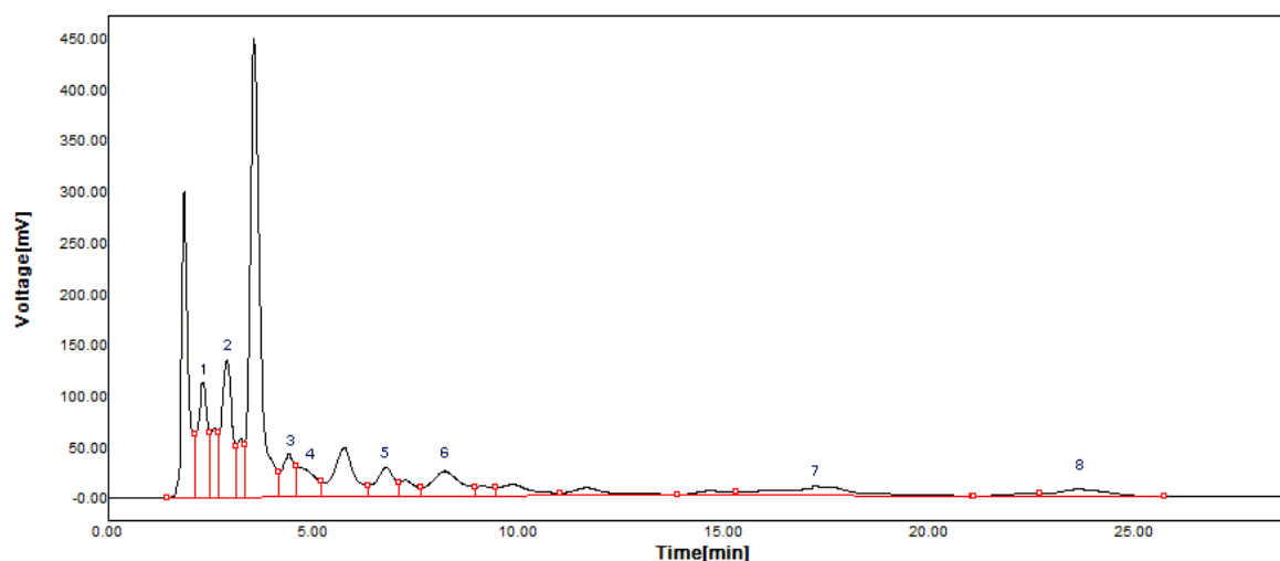
Fig. 1. Chromatogram of A. graveolens seed extracts (sample G)
