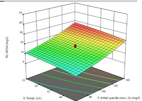
Fig. 6. 3D interaction between the adsorption parameters on R1 and the corresponding R2
