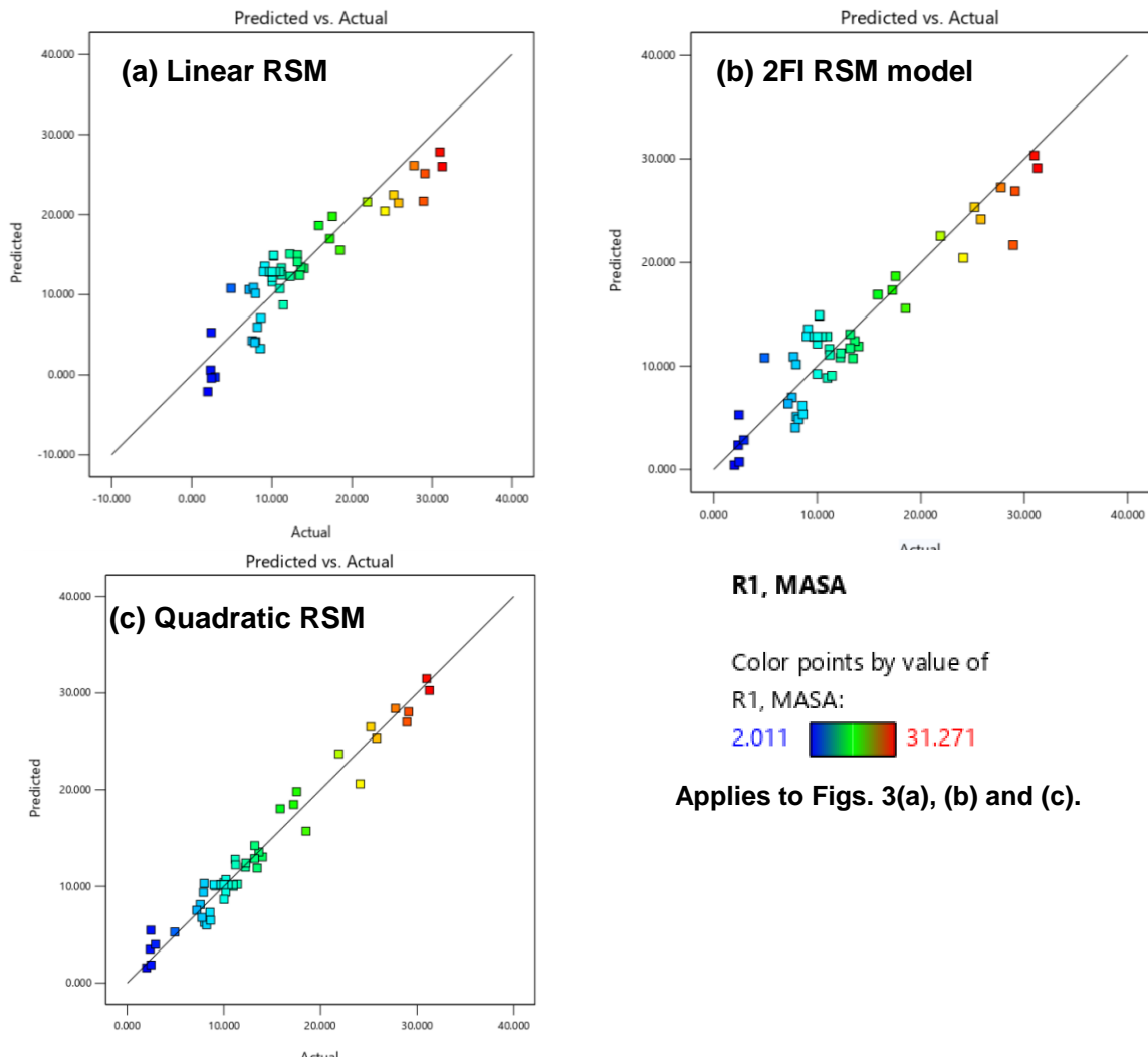
Fig. 3. Design expert software plot of actual values versus predicted values for R1 of all three RSM models studied
