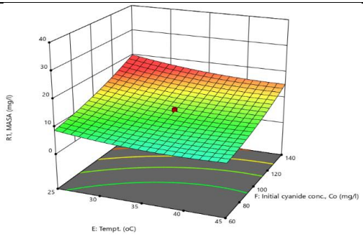
Fig. 6. 3D interaction between the adsorption parameters on R1 and the corresponding R2
