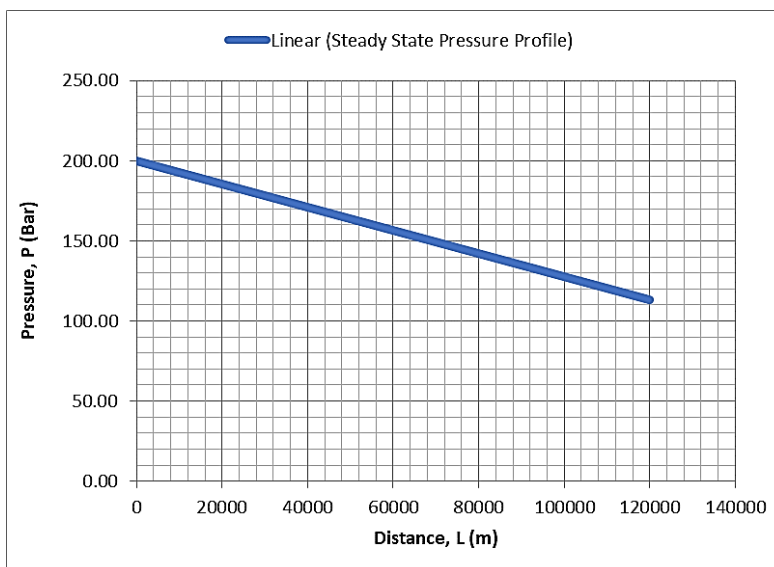
Fig. 3. Steady state pressure profile
