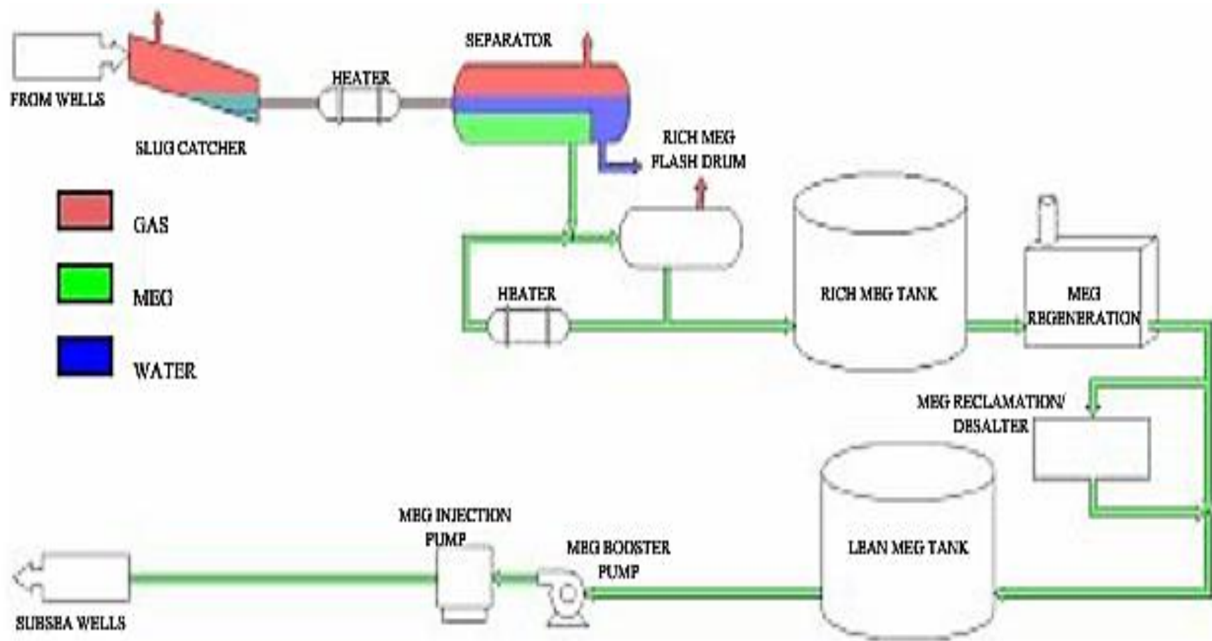
Fig. 1. Full reclamation of mono ethylene glycol [MEG] process [6]
