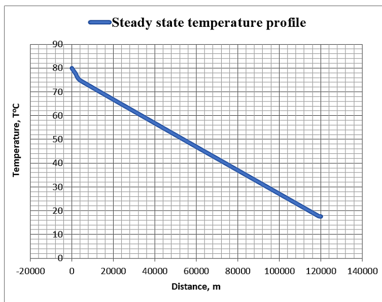
Fig. 2. Steady-state temperature profile
